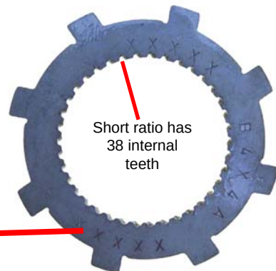
Short Ratio Star Washer Has 38 Teeth
