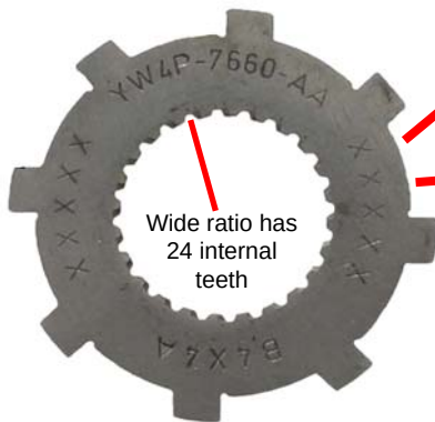
Wide Ratio Star Washer Has 24 Teeth
